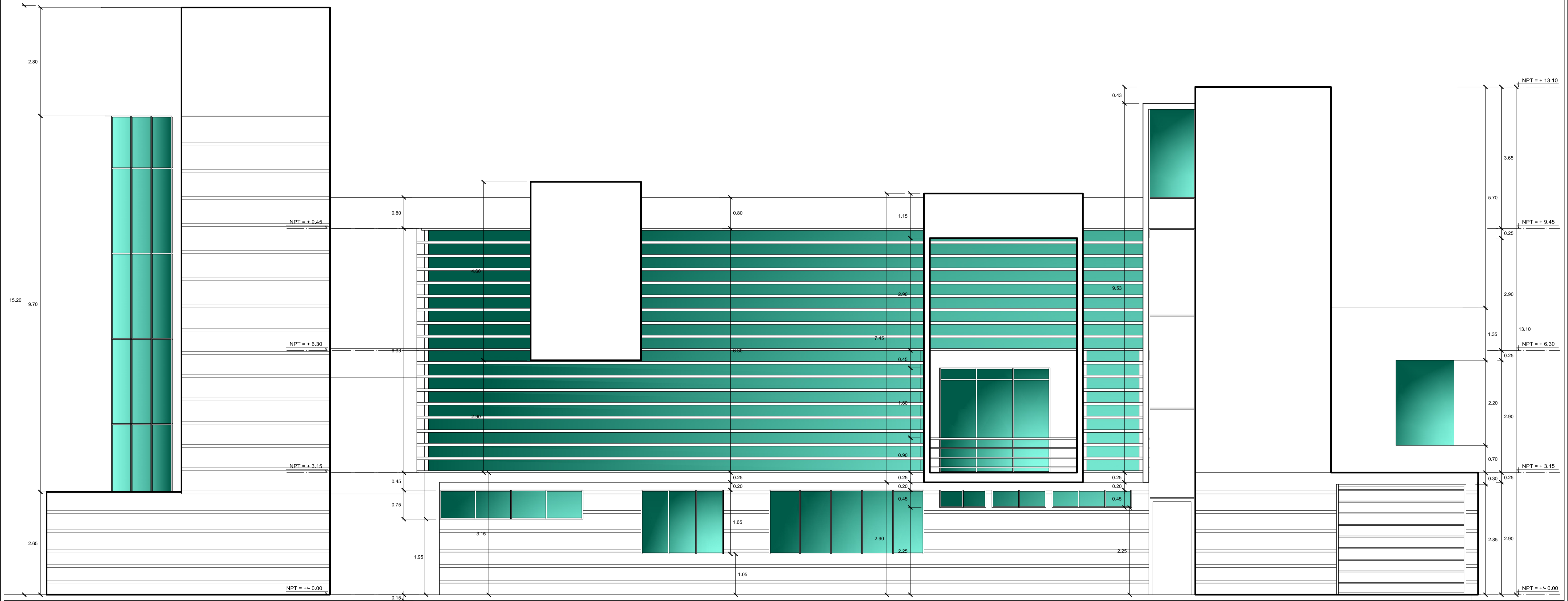
ELEVACION PRINCIPAL E-1 esc:1/50
